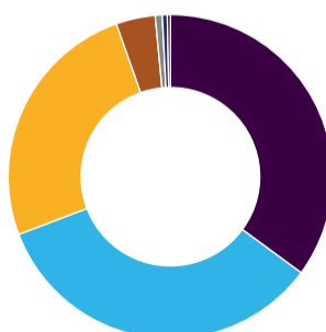
RATING ALLOCATION (2)
